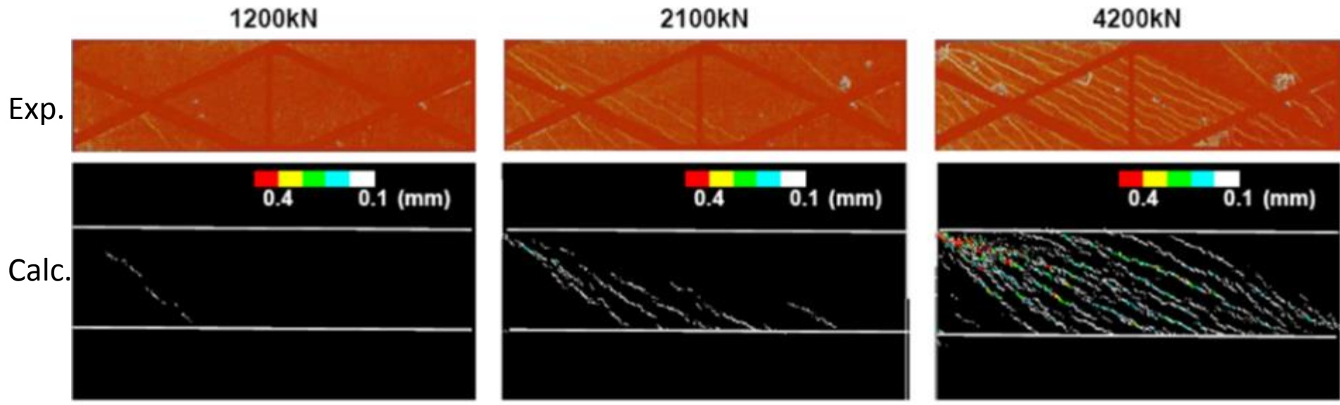
Progress of Crack pattern for different load level
